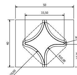
FS5040-1P WITH PEEL TAB
