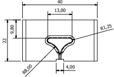
HS4022-8R WITH 5° TAPERED SIDES
