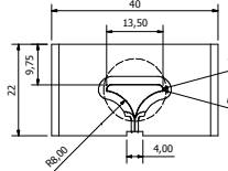
HS4022-2T WITH 5° TAPERED SIDES
